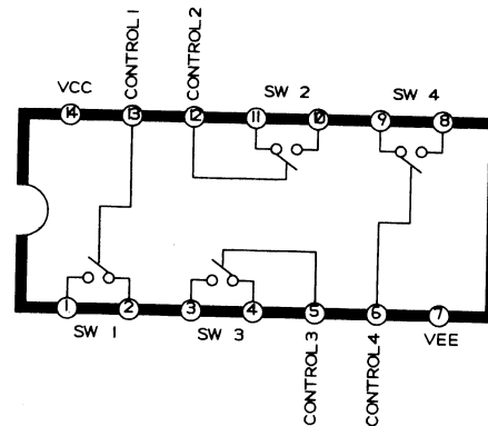
IC22 (INPUT) LC4956
