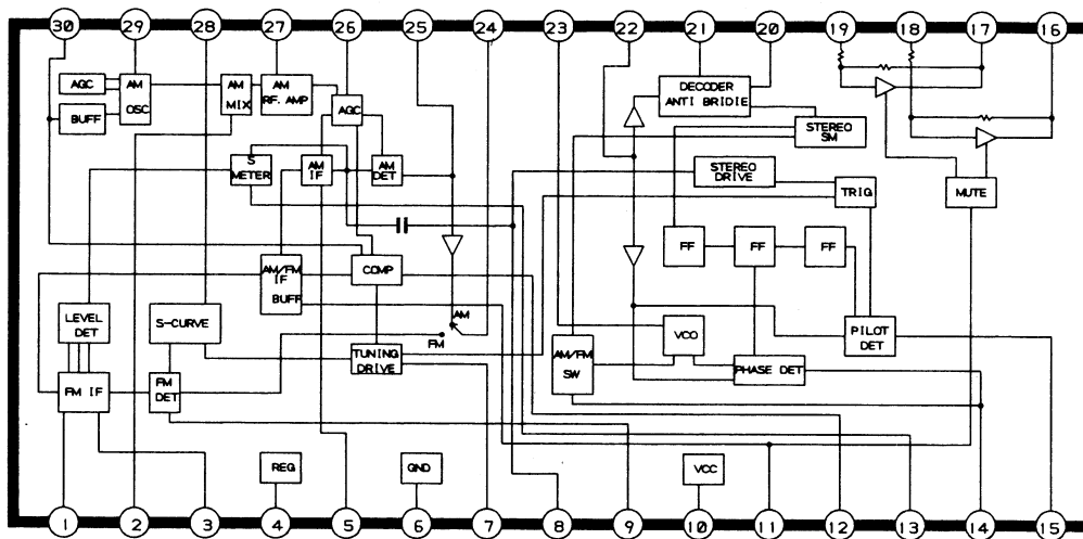
IC12 (TUNER) LA1836M BLOCK DIAGRAM
