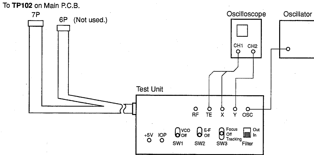
Fig. 6 Test Unit Connecting Diagram
