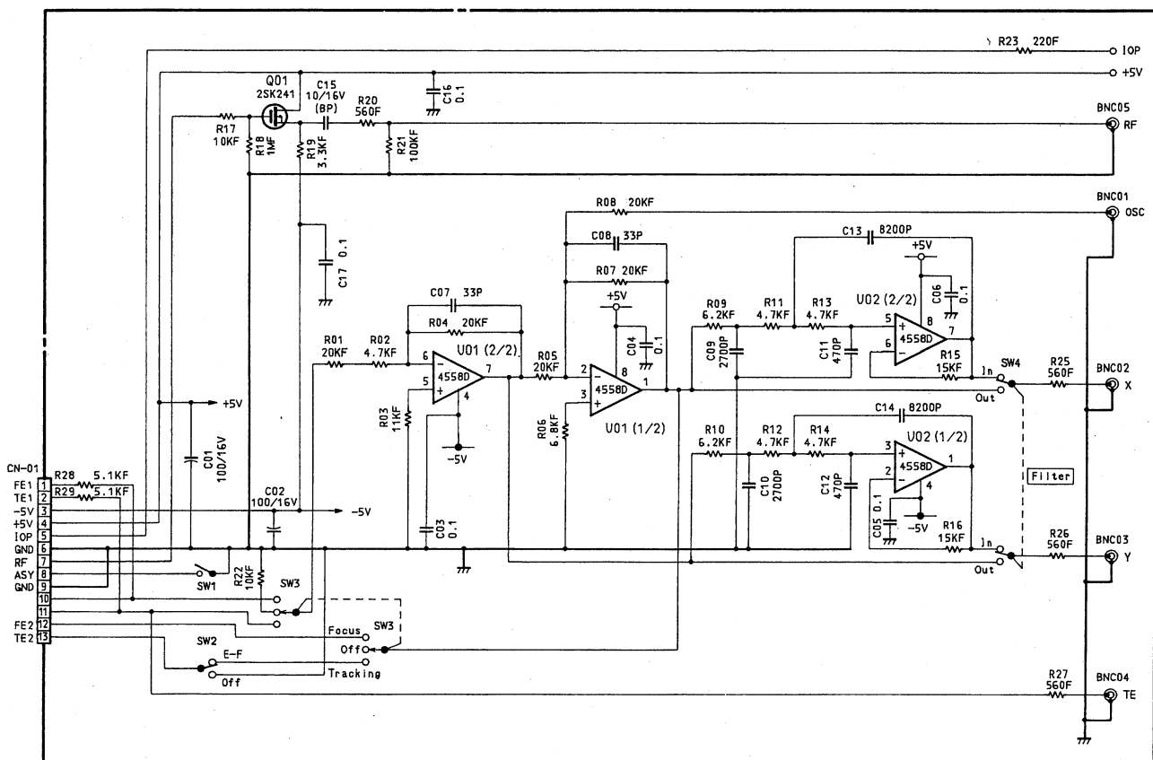
Fig. 4.2 Circuit of the Test Unit
