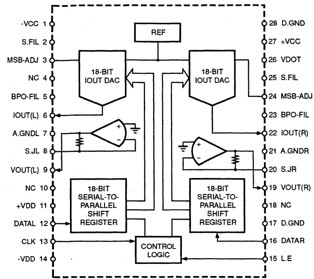
Fig. 9.7 Digital-to-Analog Converter PCM1700P (MB-1s)
