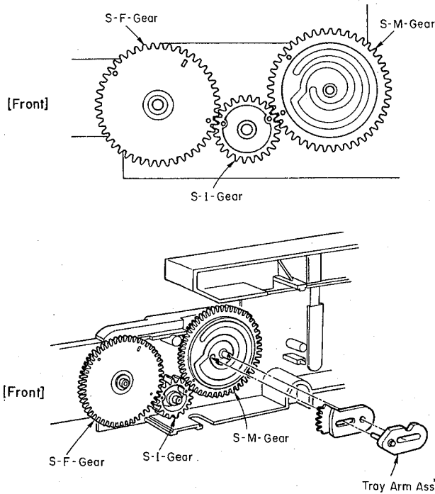
Fig. 3.1.1 Positioning of Three Gears
