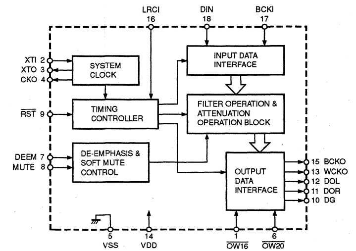
Fig. 9.8 8-Times Oversampling Digital Filter SM5841CP
