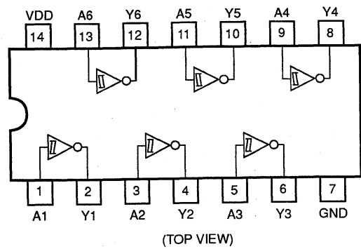
Fig. 9.1 Inverter TC4584BP
