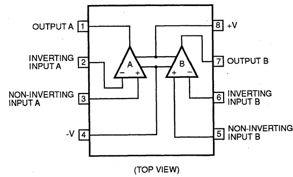
Fig. 9.4 Operational Amp. 4558D, 5532AN
