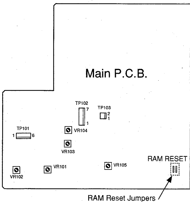
Fig. 1.2 Sticker Operation Check at Power ON
