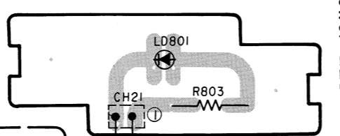
Power LED P.C. Board
