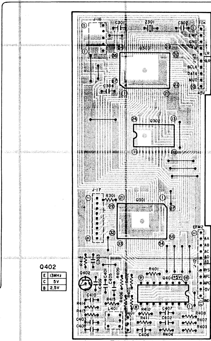
FLAT PACKAGE P.C. BOARD
